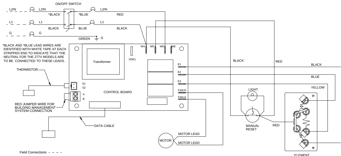
Figure 3 - Wiring Diagram
